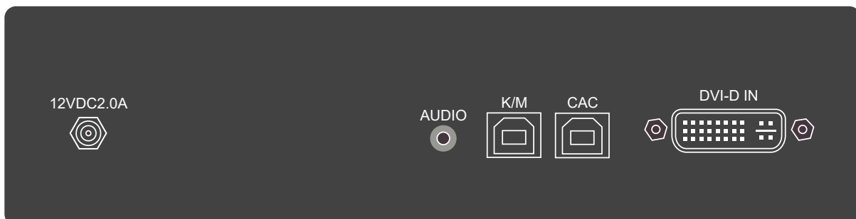
Figure 4-2: SDVN-1S-P Rear panel
