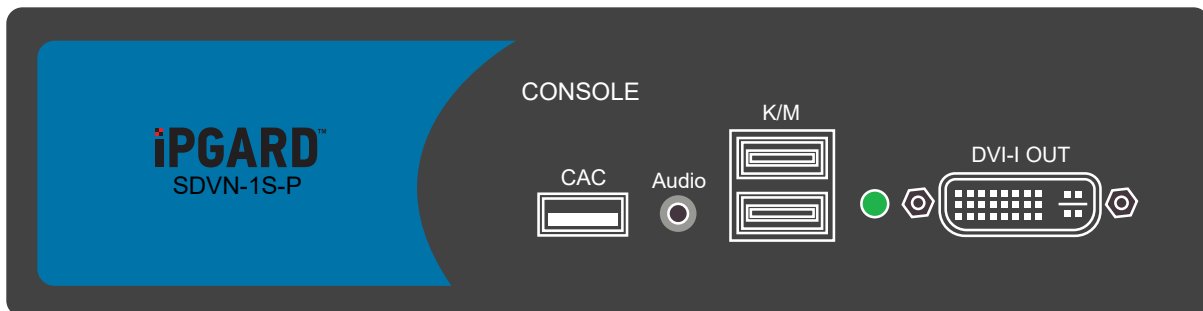
Figure 4-1: SDVN-1S-P Front panel
