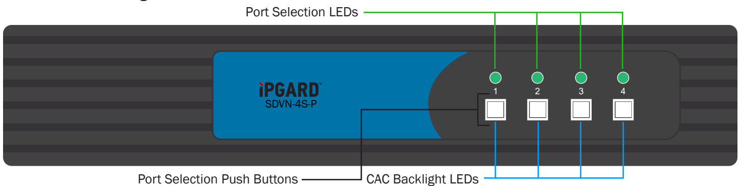
Figure 4-1: SDVN-4S-P Front panel
