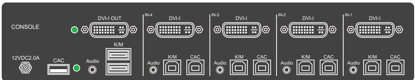
Figure 4-2: SDVN-4S-P Rear panel
