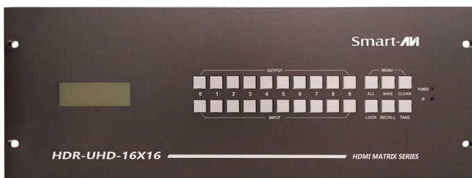
HDR-UHD-16X16 Front panel
