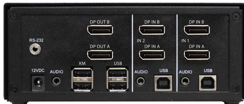
SM-DPN-2D Back
