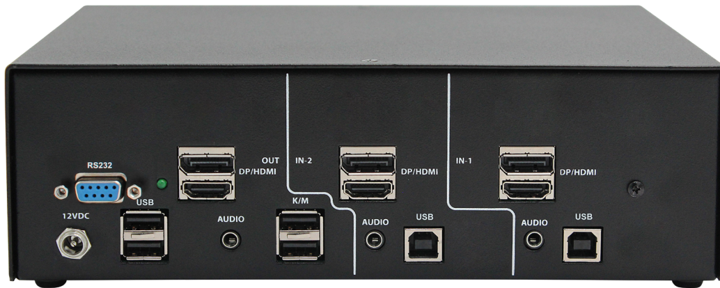
SM-UVH-2S Back panel
